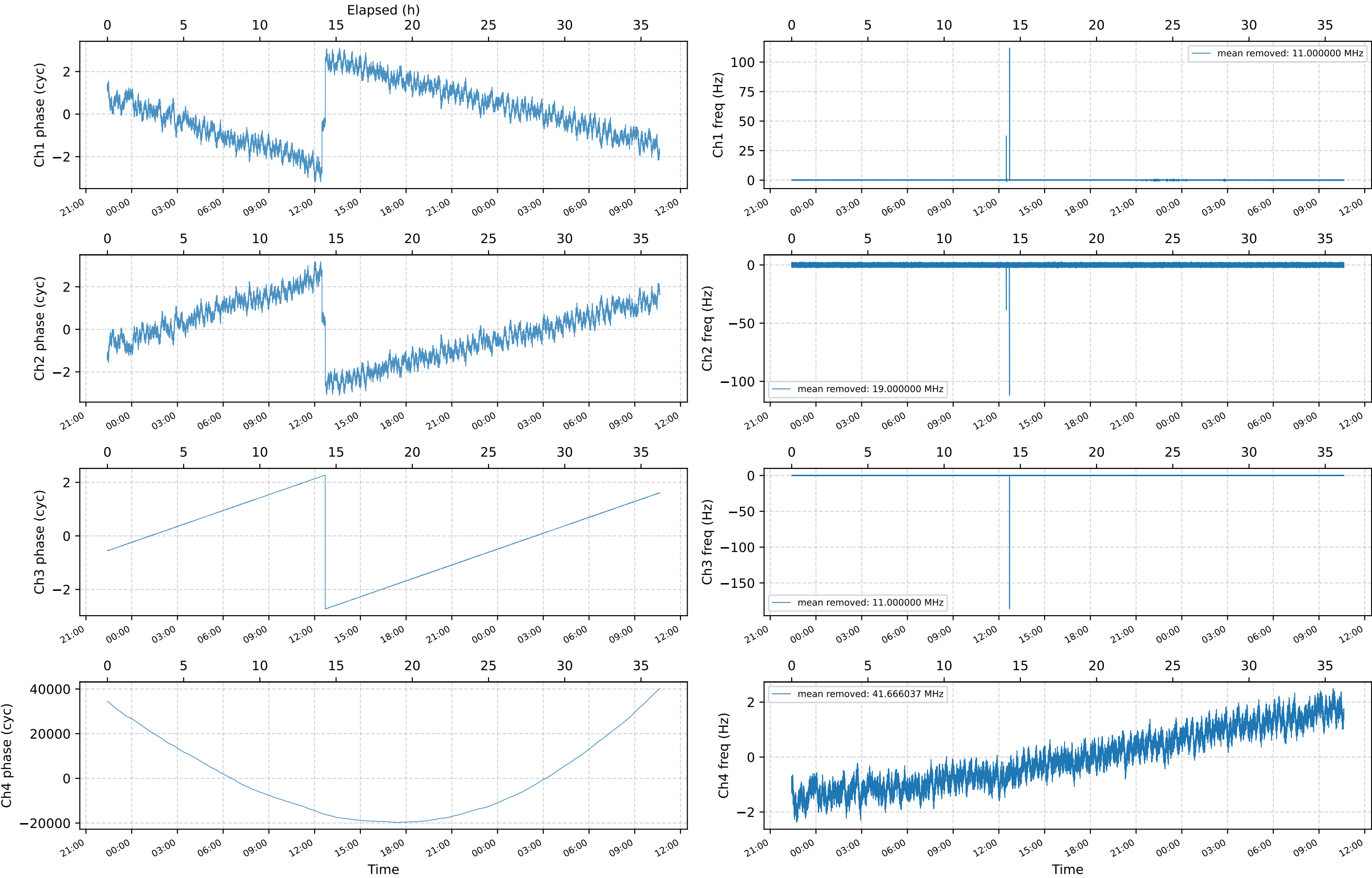
Delayline_11MHz_mix_UNDEL_DDS_400mVpp_ADC_on_inputs_1_2_and4_20260419_222428
